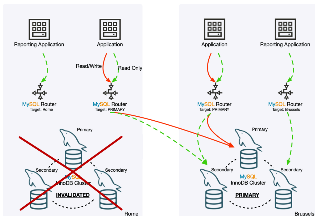
Figure 9.3 InnoDB ClusterSet Failover
